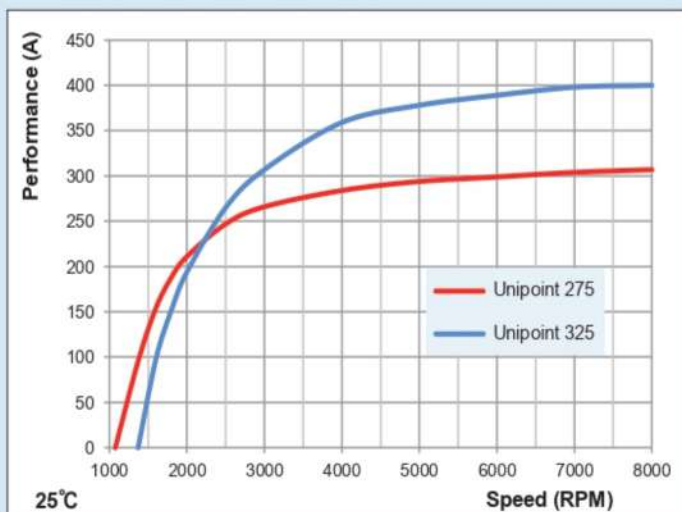
Performance Chart for 275A & 325A
